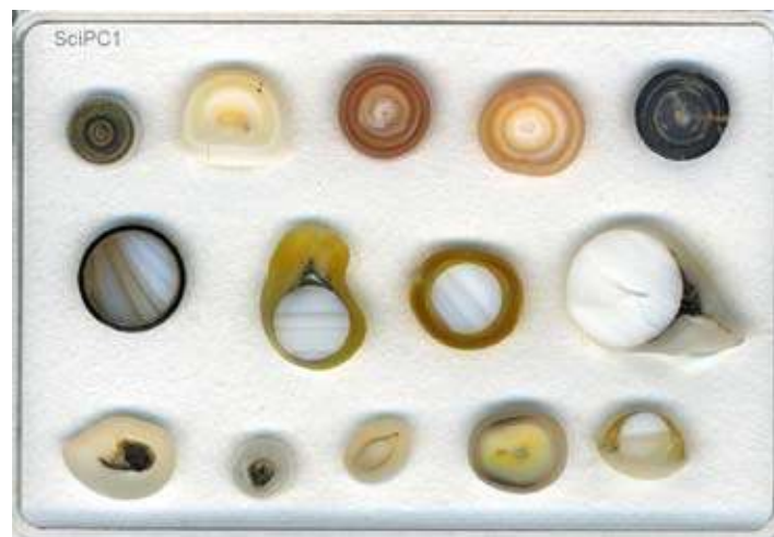
Collection of cross sections of natural pearls and cultured pearls (beaded and beadless) to study internal features of pearls. © H.A. Hänni, SSEF 2008.
