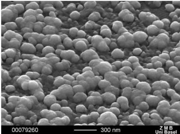
High magnification SEM picture of the surface of a coated CZ. Picture Marcel Düggelin, ZMB
